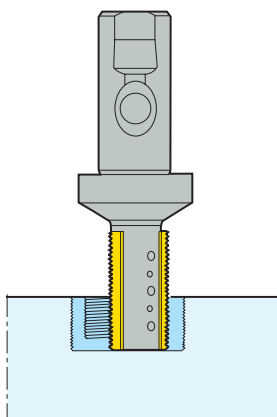
Ø 17-58 mm (0.669-2.283") Thread milling cutters with indexable inserts
