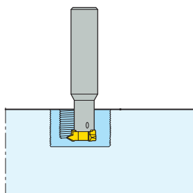
Ø 11,7-27,7 mm (0.461-1.091") Thread milling cutters with changeable head
