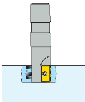
Ø 12 mm (0.472") Thread milling cutters with indexable insert
